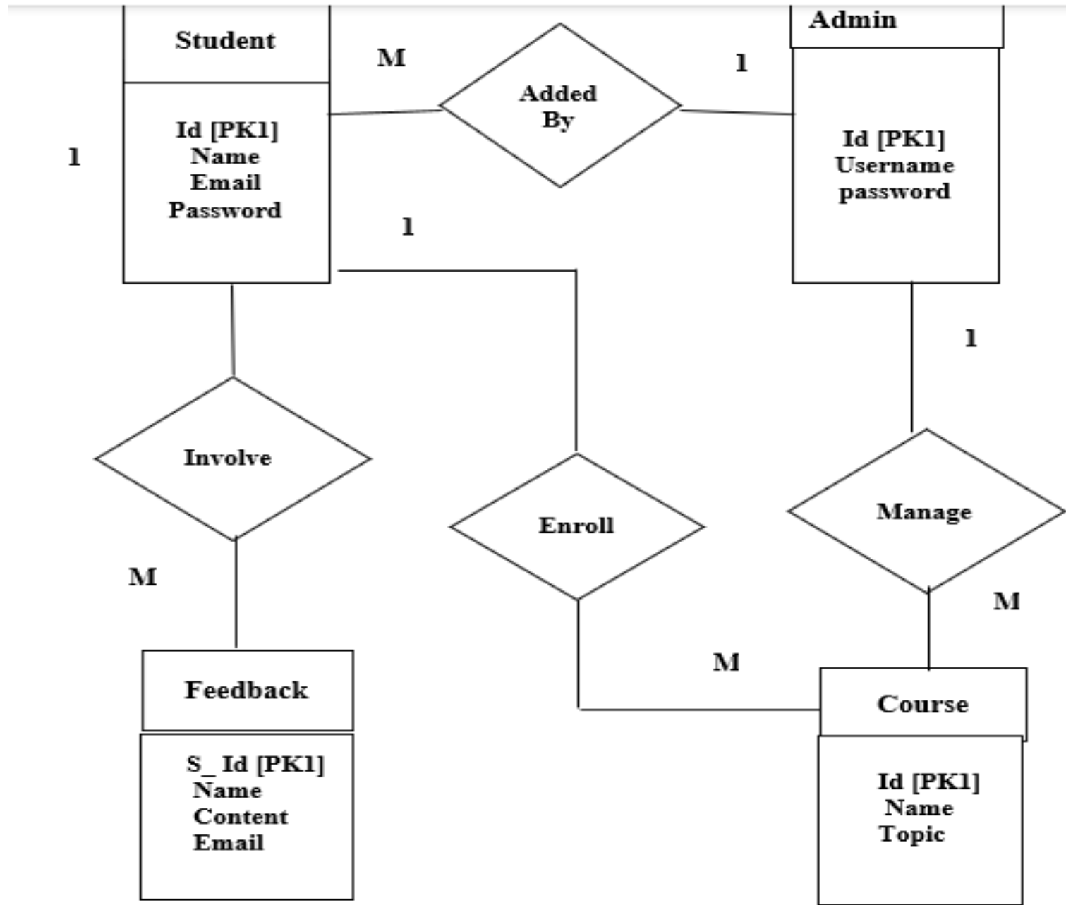
Figure: ER- Diagram for E-Learning Management System
